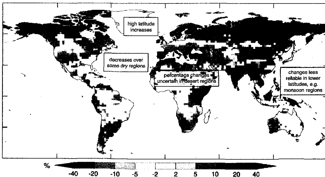
Figure 3.5. Large-scale relative changes in annual runoff (water availability, in percent) for the period 2090-2099, relative to 1980-1989. Values represent the median of 12 climate models using the SRES A1B scenario. White areas are where less than 66% of the 12 models agree on the sign of change and hatched areas are where more than 90% of models agree on the sign of change. The quality of the simulation of the observed large-scale 20 th century runoff is used as a basis for selecting the 12 models from the multi-model ensemble. The global map of annual runoff illustrates a large scale and is not intended to refer to smaller temporal and spatial scales. In areas where rainfall and runoff is very low (e.g. desert areas), small changes in runoff can lead to large percentage changes. In some regions, the sign of projected changes in runoff differs from recently observed trends. In some areas with projected increases in runoff, different seasonal effects are expected, such as increased wet season runoff and decreased dry season runoff. Studies using results from few climate models can be considerably different from the results presented here. (WGII Figure 3.4, adjusted to match the assumptions of Figure SYR 3.3; WGII 3.3.1, 3.4.1, 3.5.1)
